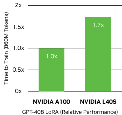
GPT-408 LoRA (Relative Performance)
